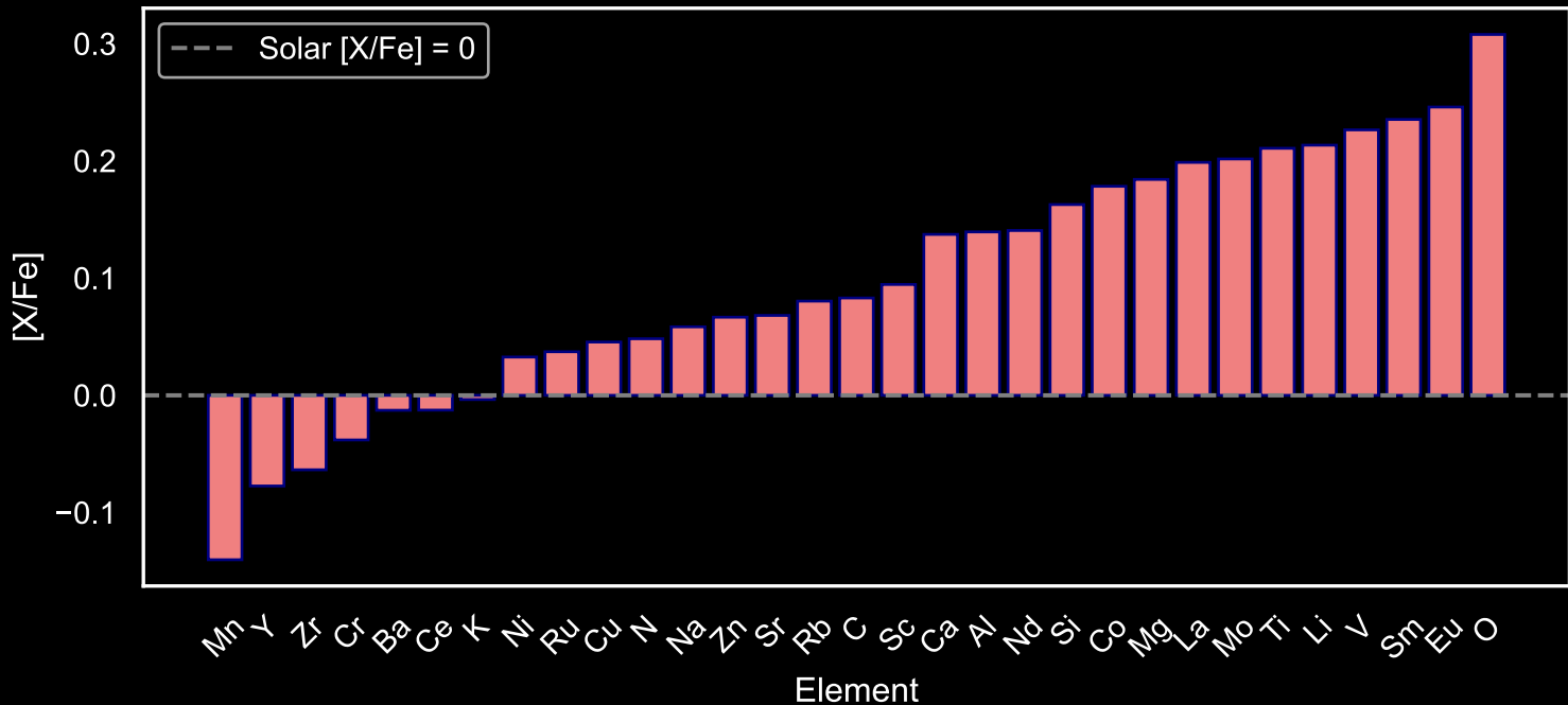
Abundance Pattern for GALAH Red Giants: Star Field [32] (N=71)
