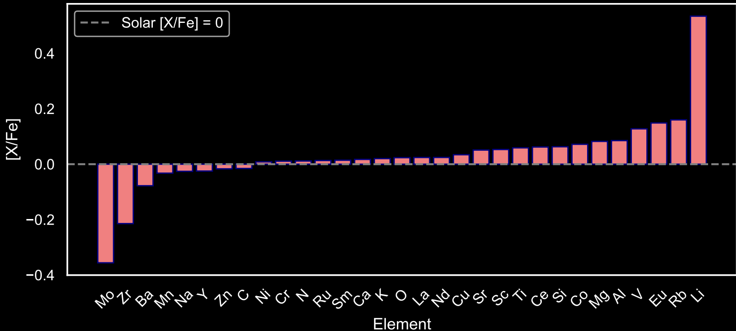
Abundance Pattern for GALAH Main Sequence Stars: Star Field [32] (N=120)
