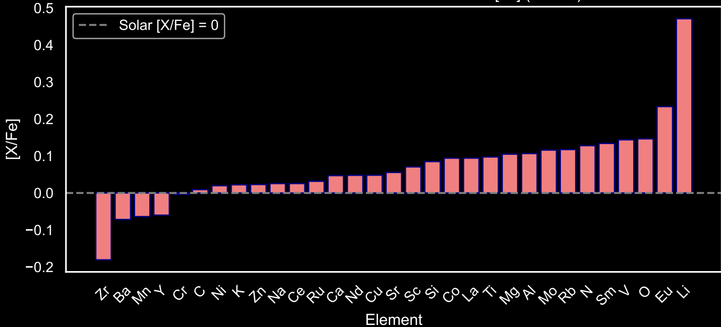
Abundance Pattern for GALAH Star Field [32] (N=262)
