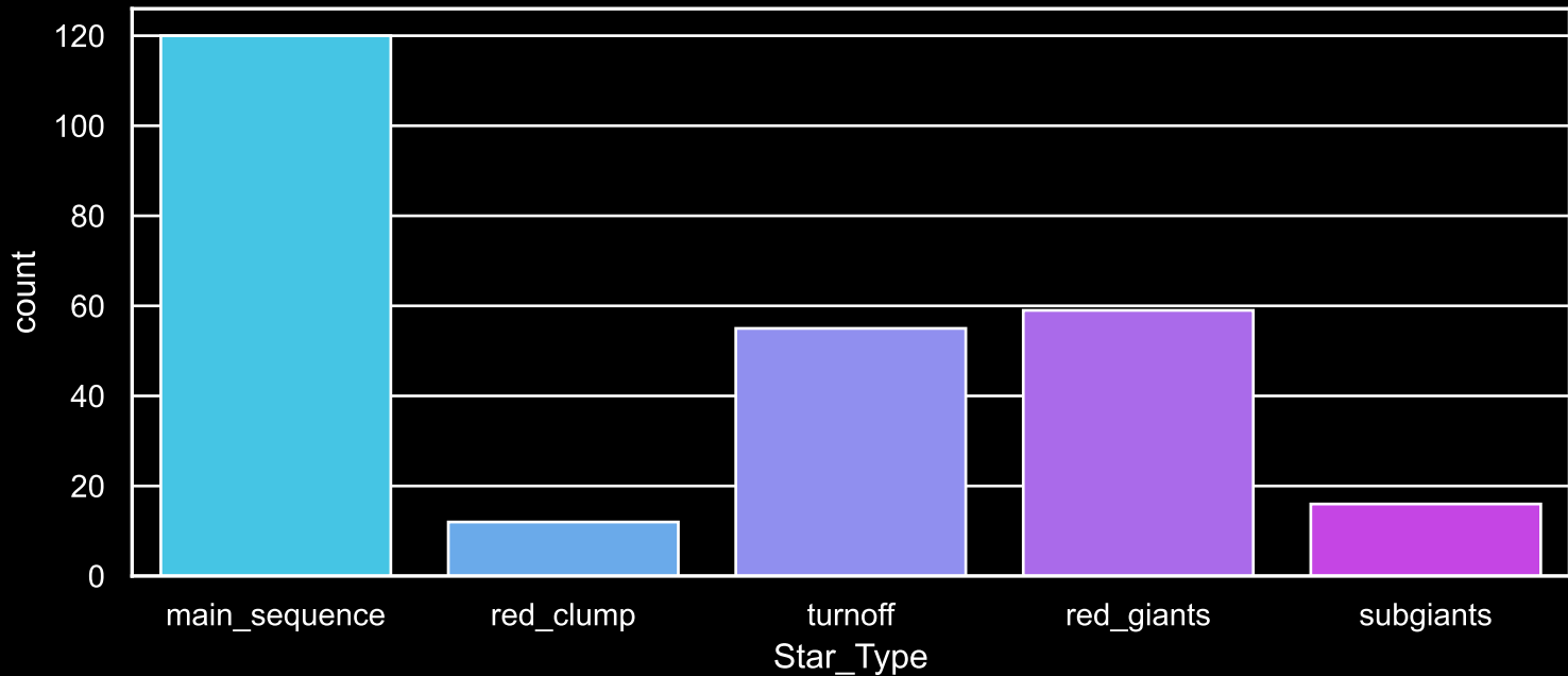
Field [32] Count plot of Star Type
